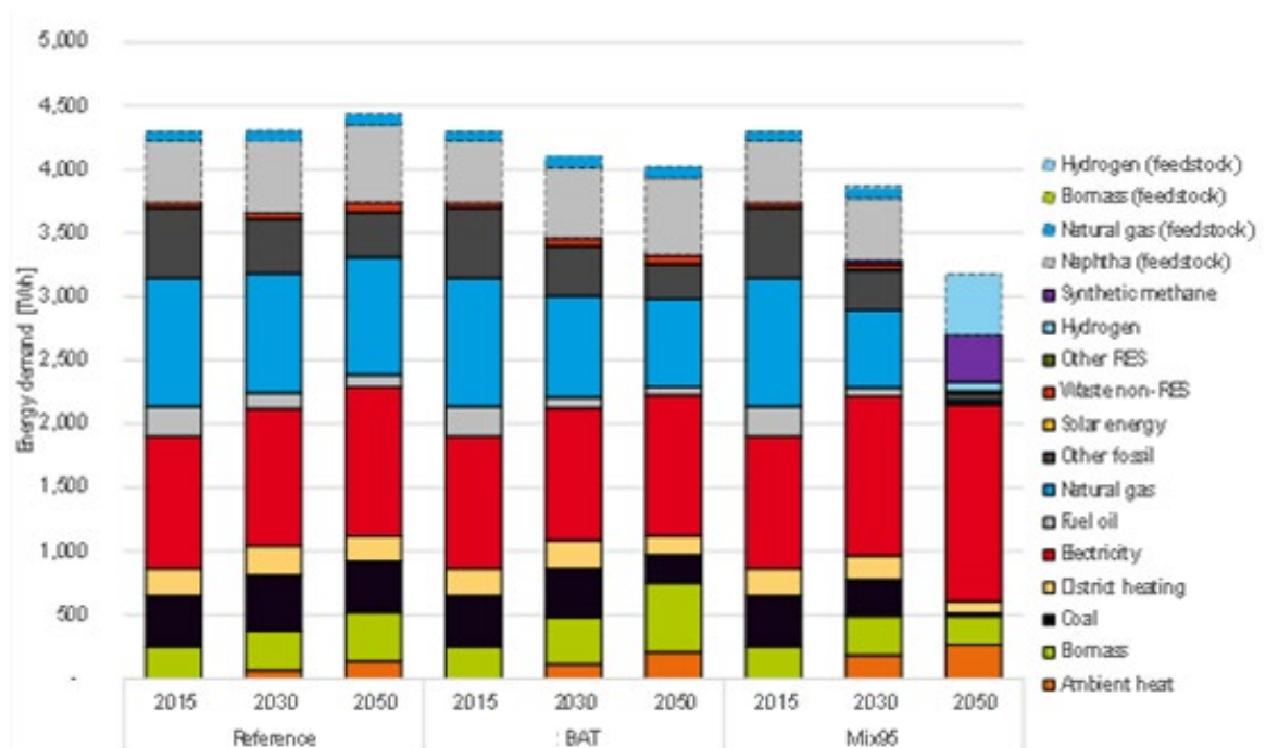
Figure 3: EU28 Final energy demand plus feedstock demand by source
