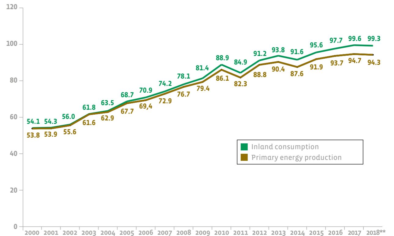
Solid biomass primary energy production and inland consumption* growth figures for the EU since 2000 (in Mtoe)
